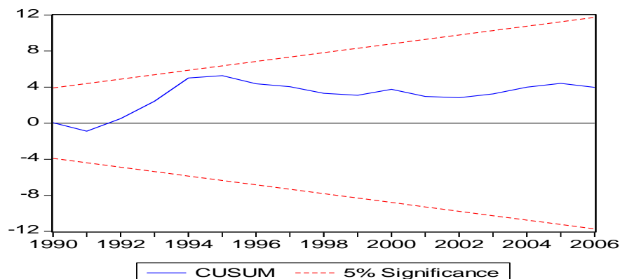
Fig. 1: Plot of Cumulative Sum of Recursive Residuals.
