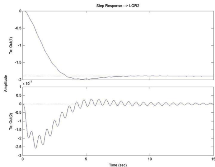
Fig. 4: Output responses to step input with optimal controllers
