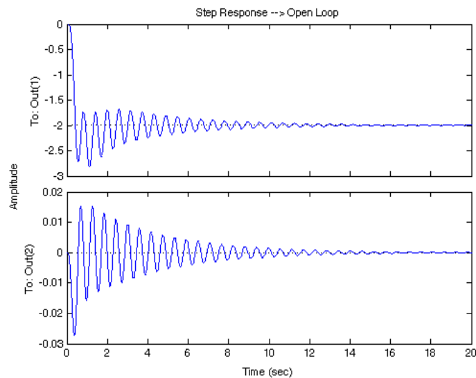
Fig. 3: Output responses to step input for open loop case
