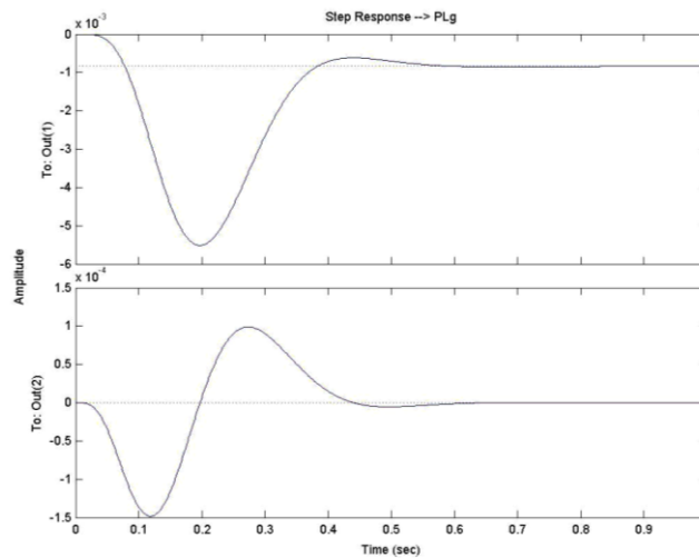
Fig. 5: Output responses to step input with state feedback controller
